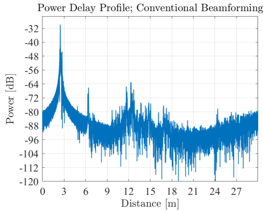
Fig. 7: Conventional wideband PDP in direction of cylinder.
